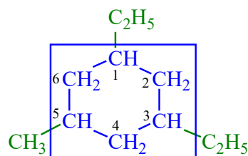
1,3-dietyl-5-metilciklohexán
